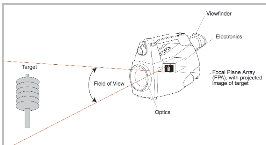
Figure 1: Overview of IR camera components. The lens focuses the target image on the photosensitive pixel elements of the FPA, which react by changing the electrical signal they send to the electronics. A 320 x 240 element FPA has 76,800 such elements. The electronics of high-performance cameras can scan each element 60 times a second, or 60 Hz, integrate the signals to produce a thermographic image, and save the data in memory.
